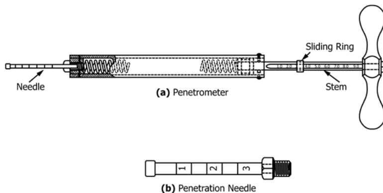
FIG. 1 Soil Penetrometer
