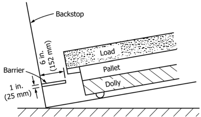
FIG. 11 Hazard Used for Fork-Tine Tip Impact Resistance
