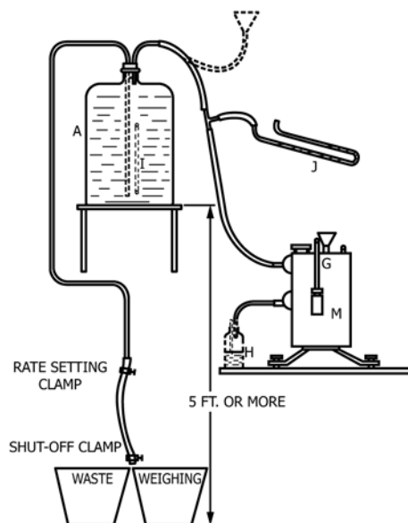
FIG. 6 Simple Equipment for Calibration by Aspirator Method
