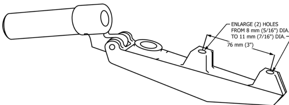
FIG. X2.1 Schematic of Modified Vacuum Pick-Up Nozzle
