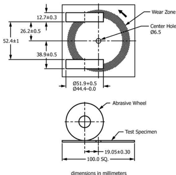
FIG. X1.1 Diagrammatic Arrangement of Taber Abraser Test Set-up
