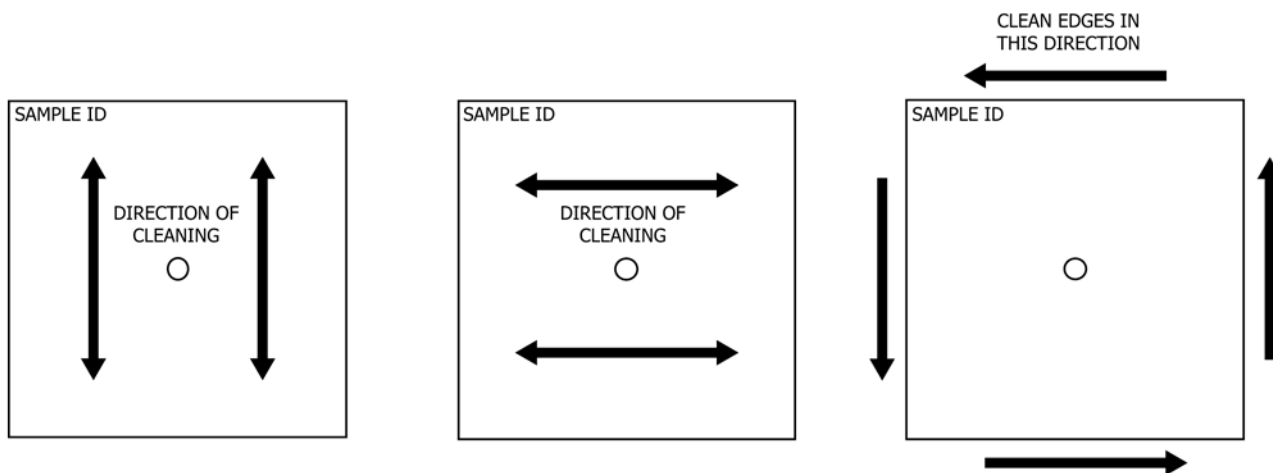
FIG. 4 Specimen Cleaning
