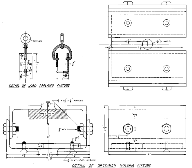
FIG. 14 Details of Testing Equipment for Measuring the Resistance of Nails to Direct Withdrawal
