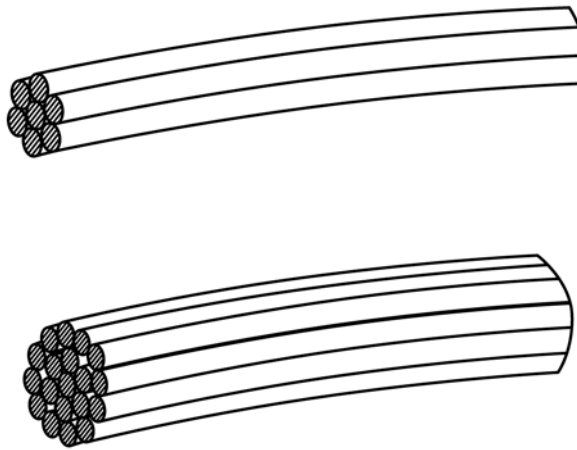
FIG. X2.1 Code 0 Illustration
