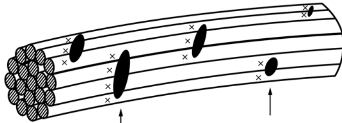
FIG. X2.5 Code 4 Illustrations
