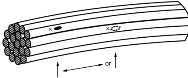
FIG. X2.2 Code 1 Illustration
