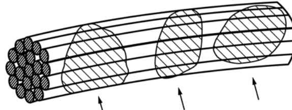
FIG. X2.6 Code 5 Illustrations
