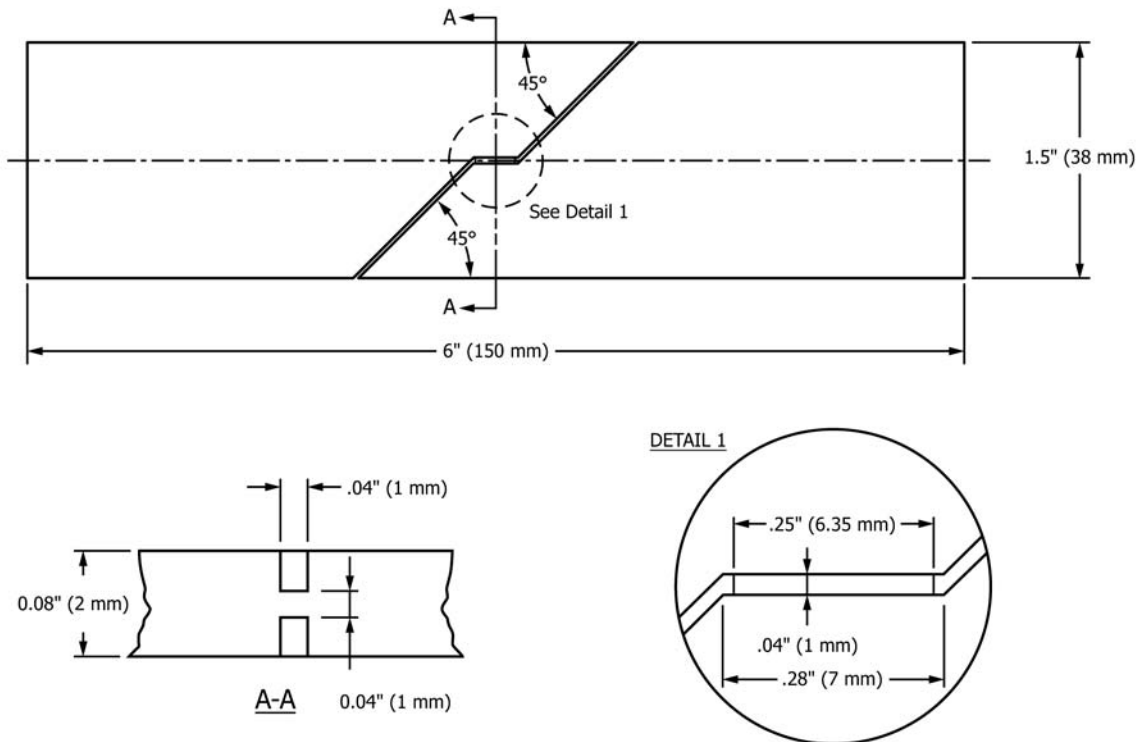
FIG. X1.1 Modified Shear Specimen
