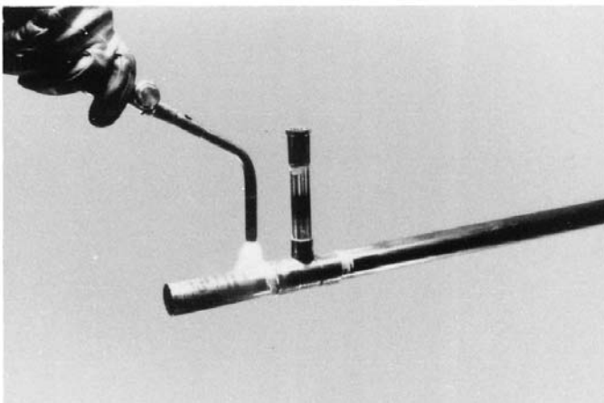
FIG. 15 Preheating: Tube
