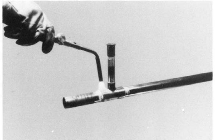
FIG. 16 Preheating: Fitting
