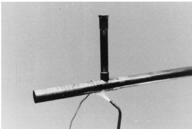
FIG. 19 Soldering
