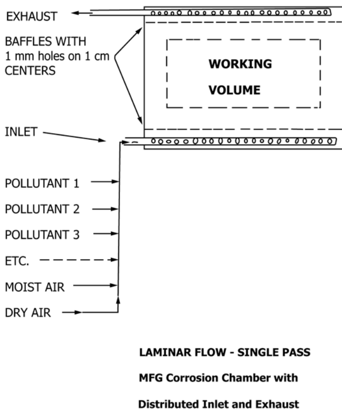
FIG. 1 Schematic Flow-Through Mixed Flowing Gas (MFG) Test System
