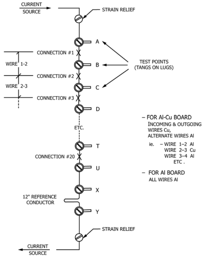
FIG. X2.2 Schematic Twist on Connector Test Board
