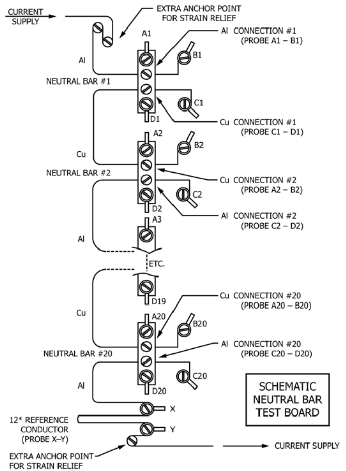
FIG. X1.2 Schematic Neutral Bar Test Board
