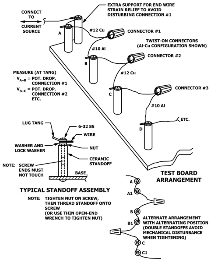
FIG. X2.1 Twist-on-Connectors
