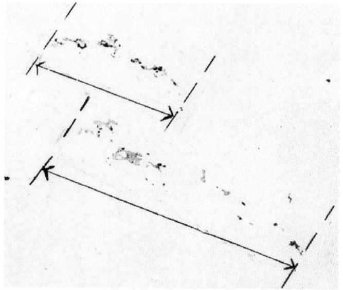
FIG. 5 Example of a discontinuous sulphide inclusion. The maximum Feret's diameter is indicated.
