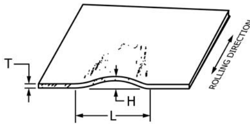
FIG. 3 Buckle
