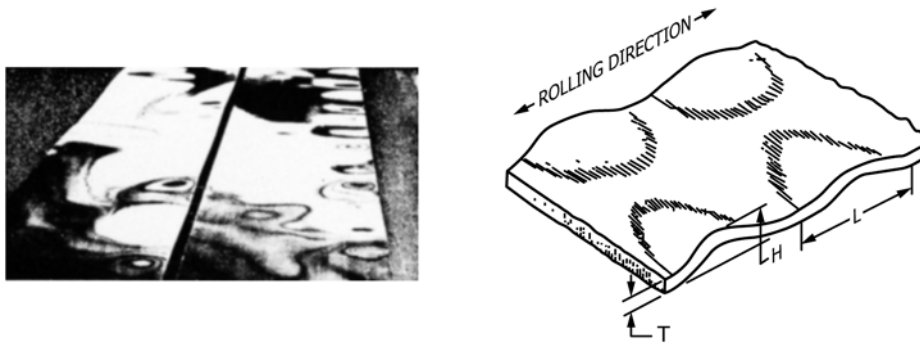
FIG. 2 Wavy Edges
