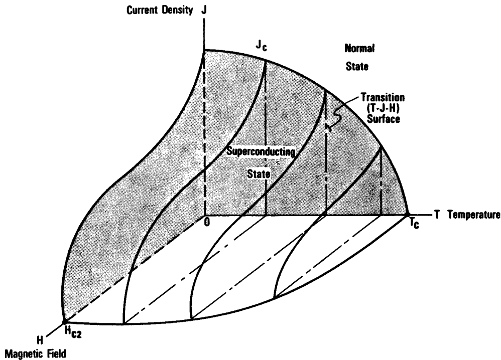
FIG. 1 Transition Surface from the Superconducting to the Normal State
