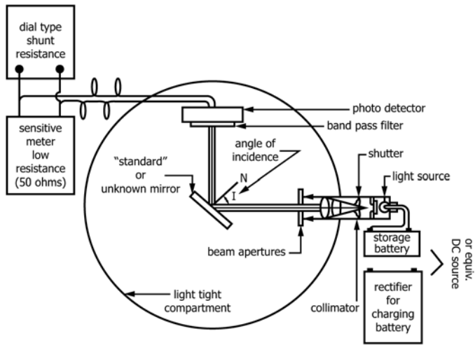
FIG. 1 Reflectivity Test
