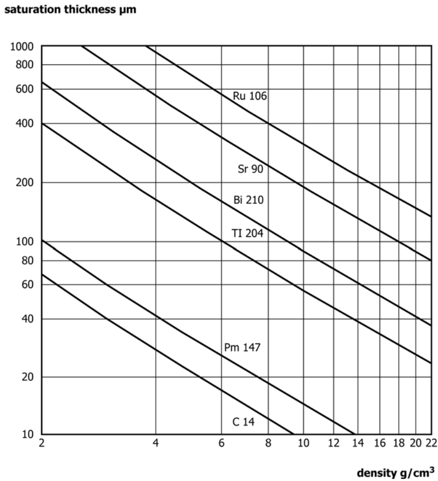
FIG. X1.1 Saturation Thickness
