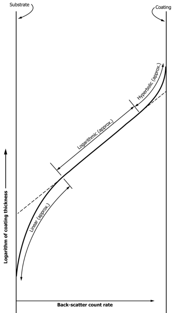
FIG. 1 Normalized Backscatter
