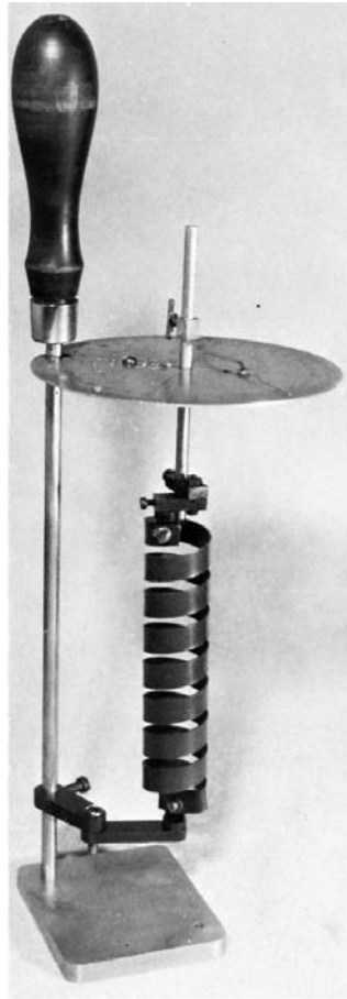
FIG. 3 Helical Coil
