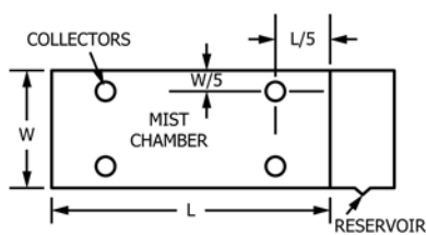
FIG. 1 Arrangement of Fog Collectors
