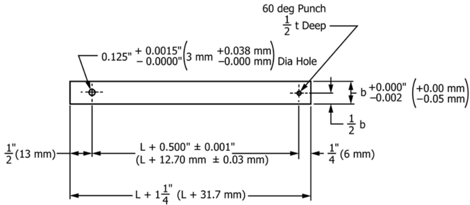
FIG. 5 Specimen
