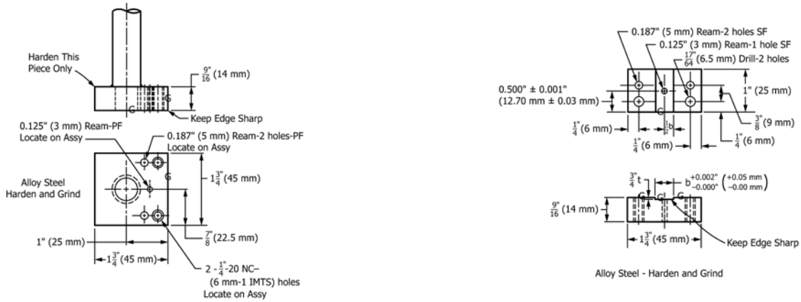
FIG. 3 Specimen Mounting Clamp Details
